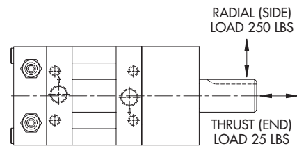
Shaft Load Capacity
